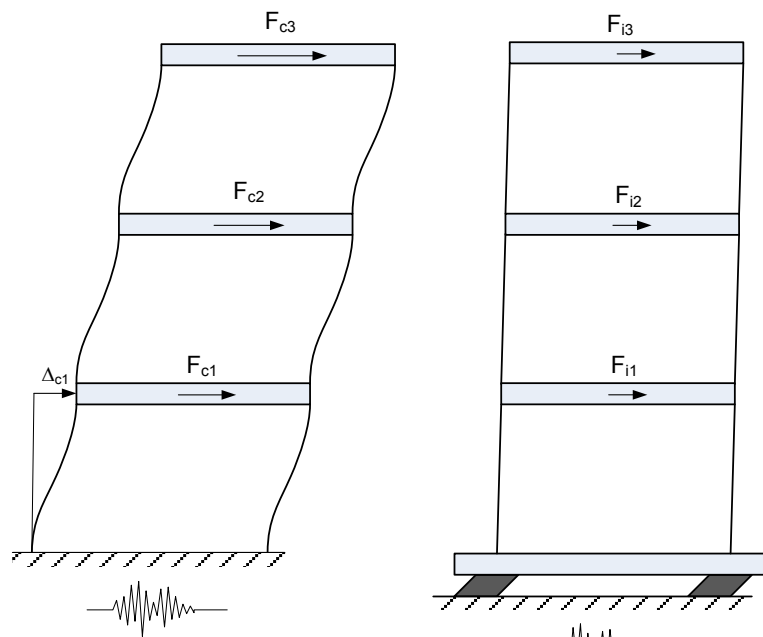
Comparison between conventional and isolated structure behaviour
